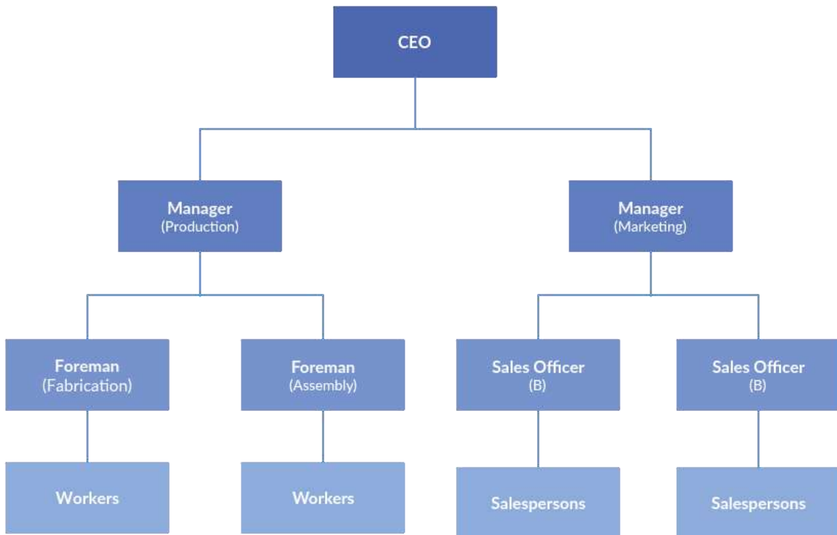
Fig 1. Hierarchical organogram
