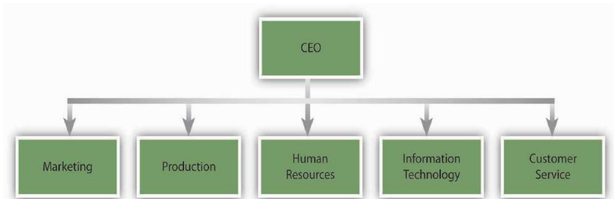
Fig 2: Flat organogram
